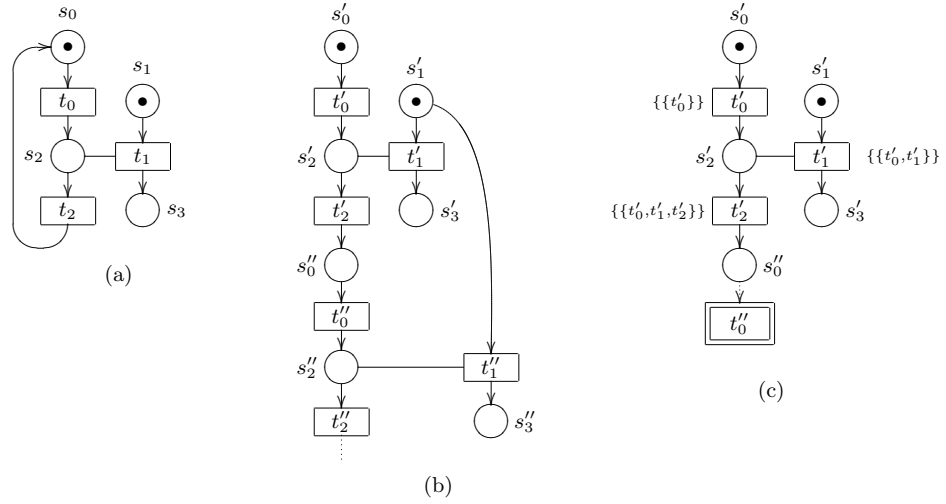
Fig. 2. (a) A contextual net N_0 , (b) its unfolding \mathcal{U}_a(N_0) and (c) a complete enriched prefix.
