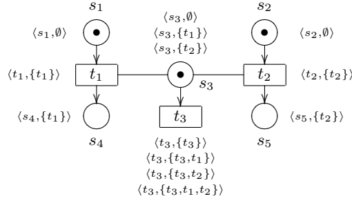
Fig. 5. Illustration of extended transitions and places
